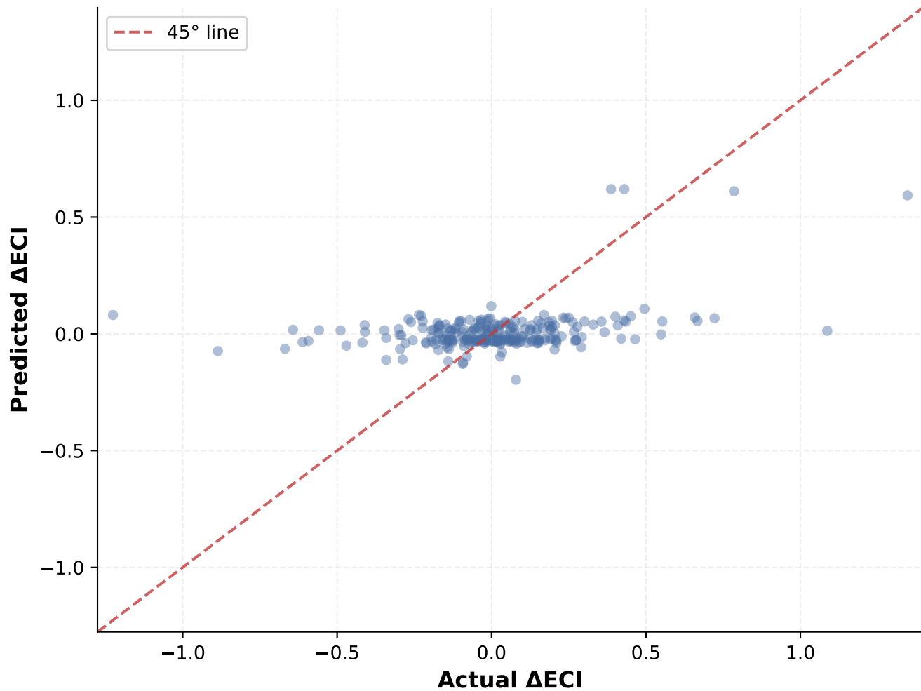
Random Forest — \Delta ECI | Test R^2=0.152 RMSE=0.2368
