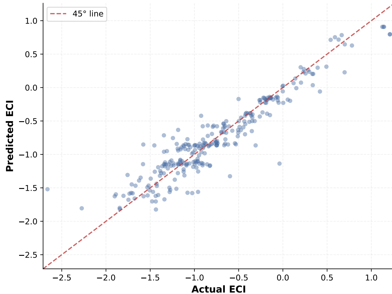
Random Forest — ECI | Test R^2=0.876 RMSE=0.2291
